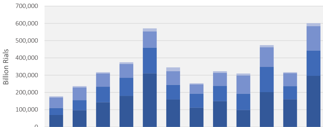
Figure 5: Annual trend of total trading value for each exchange
